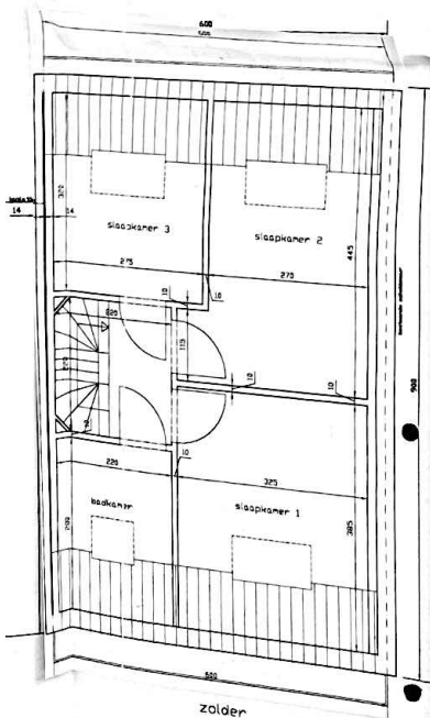
zolder
